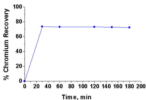
Figure 5. Chromium recovery using 5 M sodium hydroxide, solid-liquid ratio of 1/20
