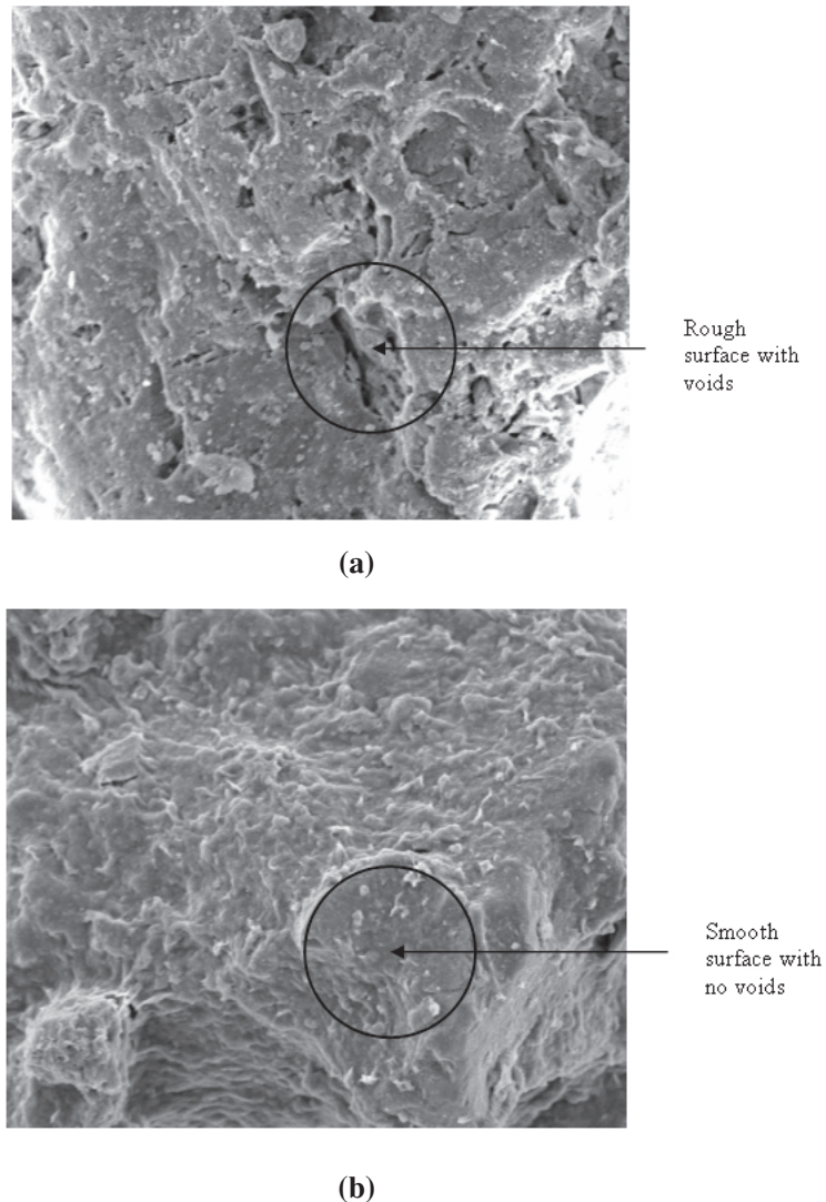
Figure 8. Scanning electron microscopy pictures with 1500 times magnification: (a) sand surface (b) sand surface with bentonite.
