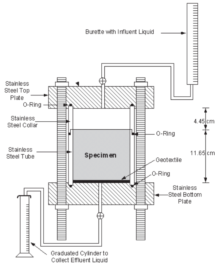
Figure 1. Rigid wall permeameter.
