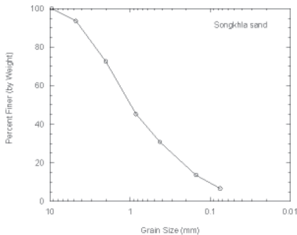
Figure 2. Grain size distribution of Songkhla sand.
