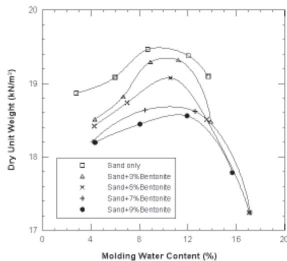
Figure 3. Compaction curves of sand-bentonite mixtures.
