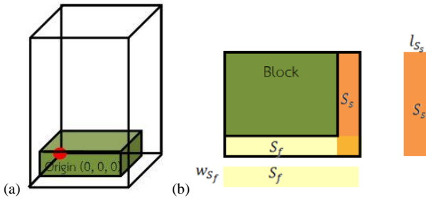
Figure 4. (a) Putting a block in R at the origin. (b) The free space on the side of block ( S_s ) and the front of block ( S_f ). W_{S_f} and l_s are width and length, respectively, of the free space on the side of block.
