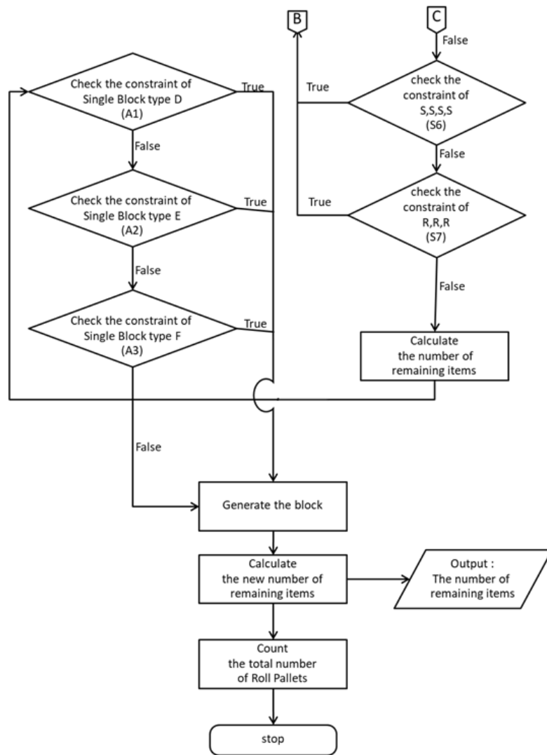
Figure 6. A flowchart of the algorithm
