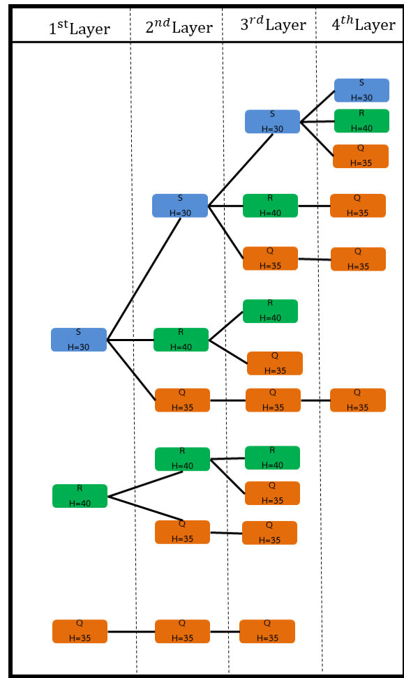
Figure 5. Tree search for all patterns on layer placement, where S, Q, R are the layer types, and H is the height of each layer (cm).
