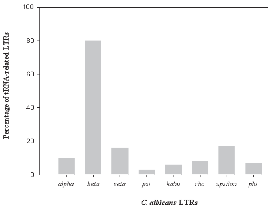
Figure 1. Inconsistent distribution of the tRNA gene-associated LTRs in C. albicans . Only beta DNA element appeared to be a hot spot harbouring the tRNA genes (see text for details).
