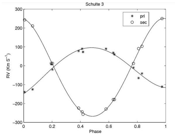
Figure 2. Radial velocities of the primary and secondary components of Schulte 3 plotted against the phase. The observational data have been measured by Kiminki et al. (2008).
