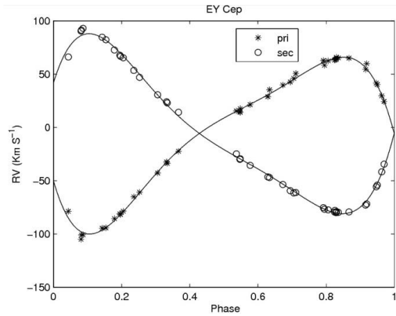
Figure 3. Radial velocities of the primary and secondary components of EY Cep plotted against the phase. The observational data have been measured by Sandberg Lacy et al. (2006).
