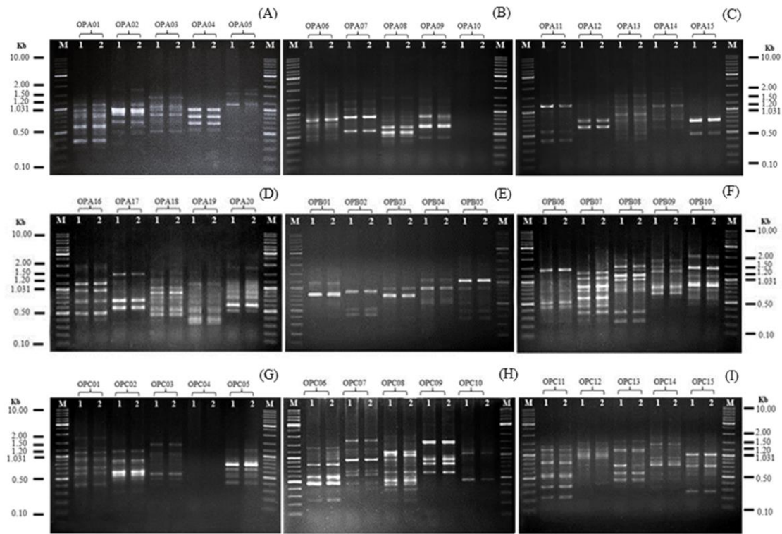
Figure 2. RAPD patterns of orchid plants raised from (1) non-cryopreserved and (2) cryopreserved protocorms of C. finlaysonianum using 45 primers: (A) primers OPA01-05; (B) primers OPA06-10; (C) primers OPA11-15; (D) primers OPA16-20; (E) primers OPB01-05; (F) primers OPB06-10; (G) primers OPC01-05; (H) primers OPC06-10; (I) primers OPC11-15.
