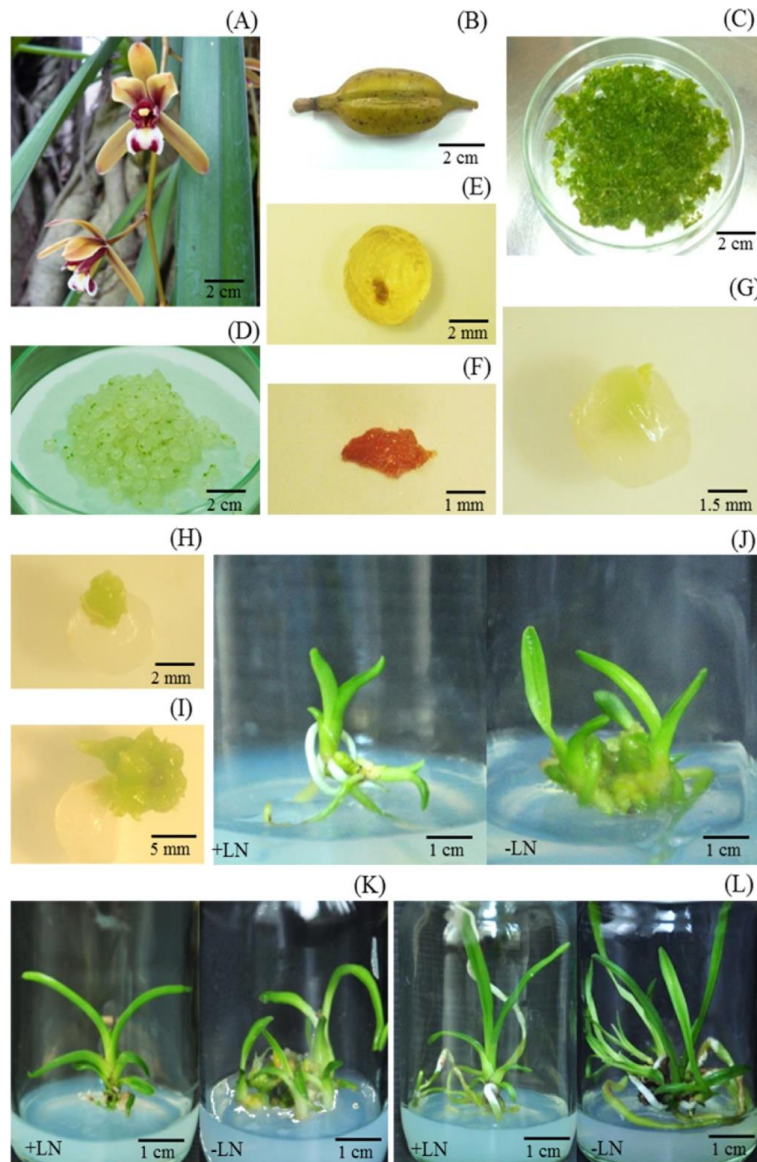
Figure 1. Cryopreservation protocols of C. finlaysonianum : (A) Flower; (B) Fruit; (C) Protocorms for cryopreservation; (D) Encapsulate beads; (E-F) TTC staining of cryopreserved beads and protocorms; (G-I) Development of cryopreserved protocorms after freezing for 1 week, 3 weeks, 8 weeks respectively; (J-L) Plantlets derived from cryo-preserved (+LN) and non-cryopreserved protocorms (-LN) for 16 weeks, 24 weeks and 36 weeks respectively. (Scale bar = 1mm-2cm)
